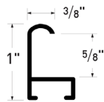
PROFILE 15
