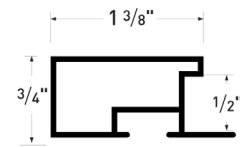
PROFILE 100
