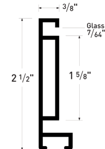
PROFILE 100
