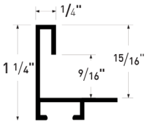
PROFILE 13
