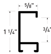
PROFILE 94
